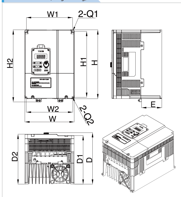
Frame 3 (weight:6.5Kg)
