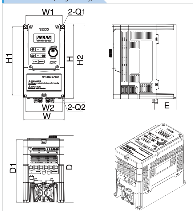
Frame 1 (weight:1.7Kg)
