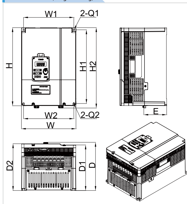
Frame 4 (weight:10.5Kg)
