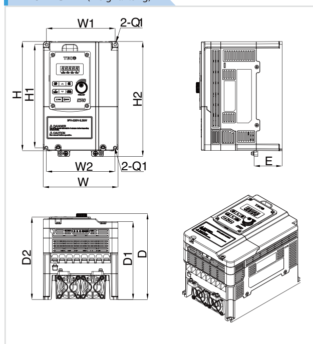
Frame 2 (weight:2.5Kg)
